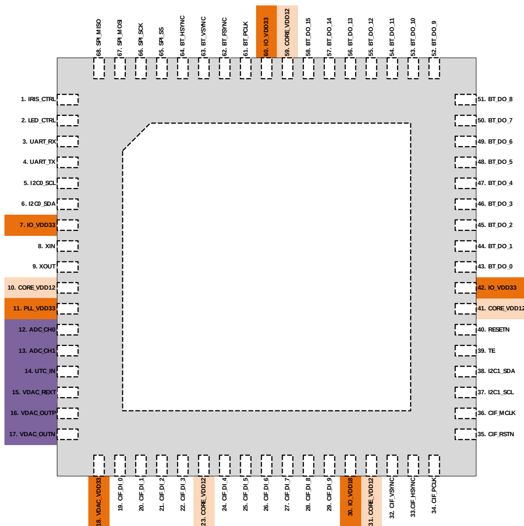
Figure 2 PI4018K Package View
